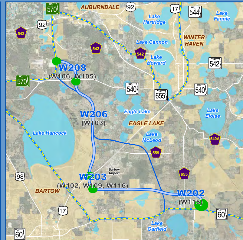
Alignment W-I
